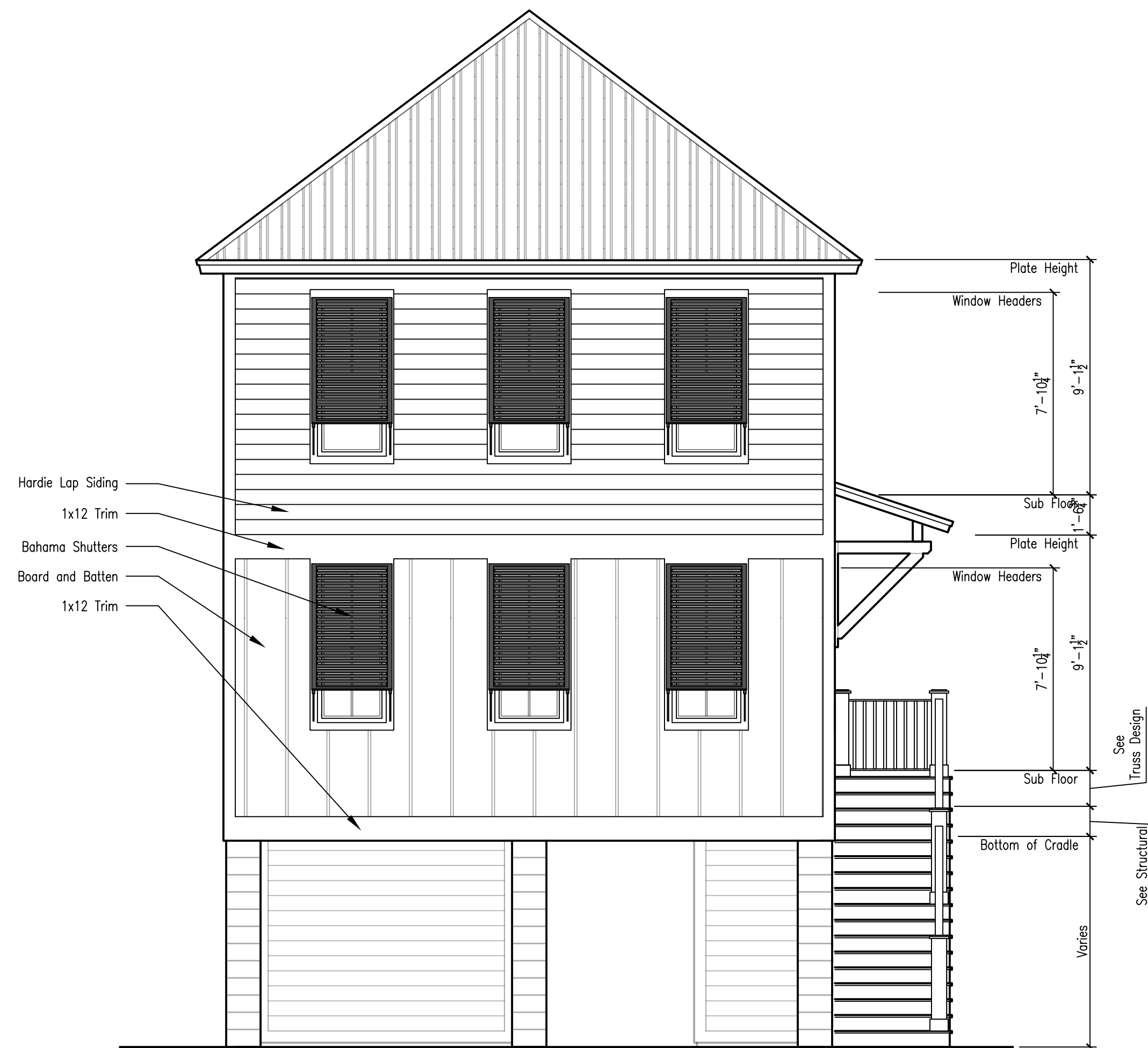
Front Elevation
